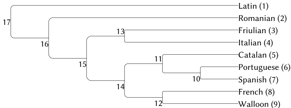
Fig 1. An example tree showing the relationships of N = 9 languages.
